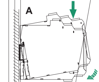
A. Snap metal lock onto mounting rail, then rotate the device, as figure A, press down the device onto mounting rail.
