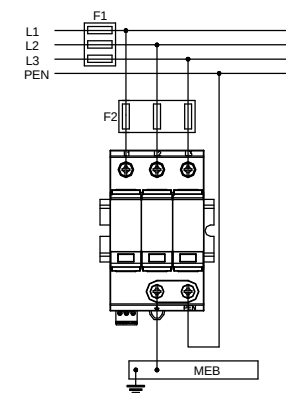
Three-phase TN-C system
