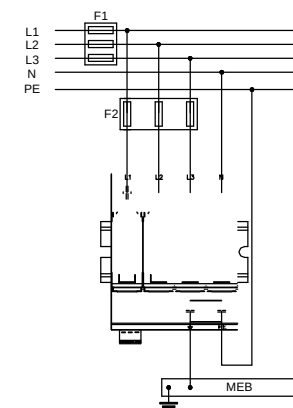
Three-phase TN-S system
